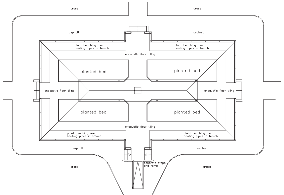
Plan as Existing 1:100
