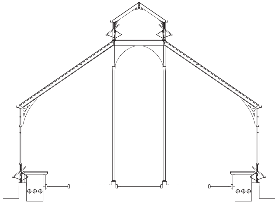
Section as Existing 1:50
