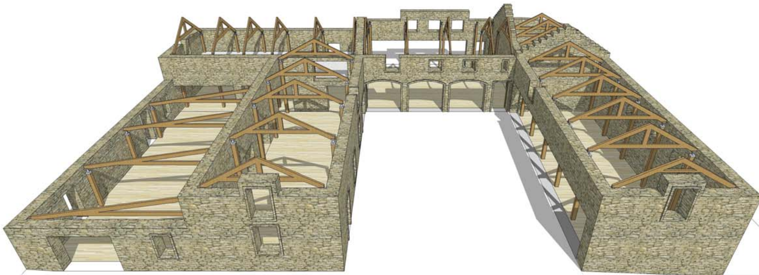
Structural Timber Frame to be constructed inside existing walls
